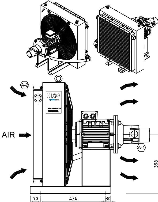
SPECIFICATION OF AIR OIL COOLER
